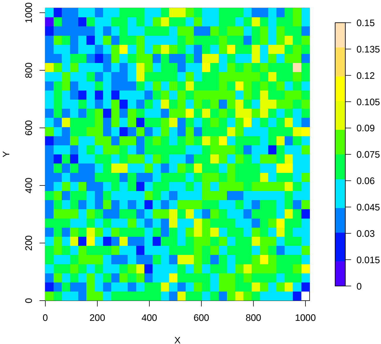
48472a OPS: binned median of "Ks - w2mpro" [mag]
