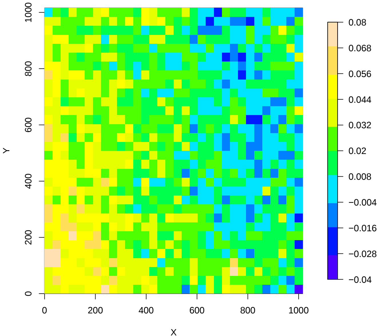
47585b POPS: binned median of "Ks - w2mpro" [mag]
