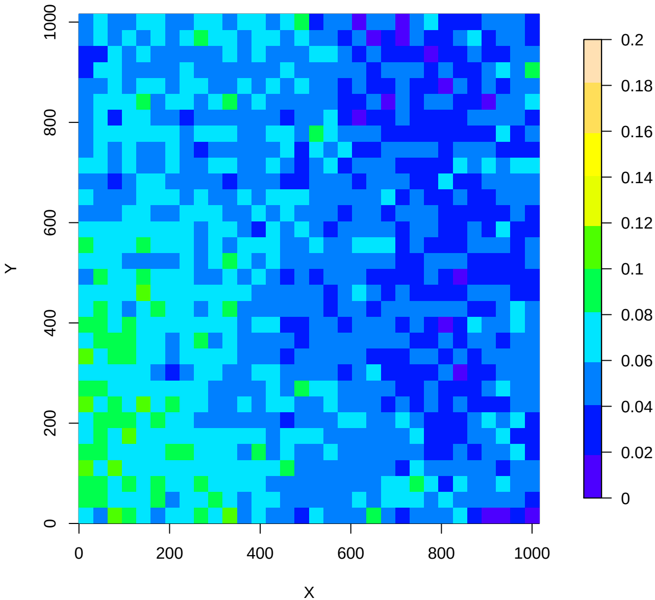
46938a: binned median of "Ks - w2mpro" [mag]
