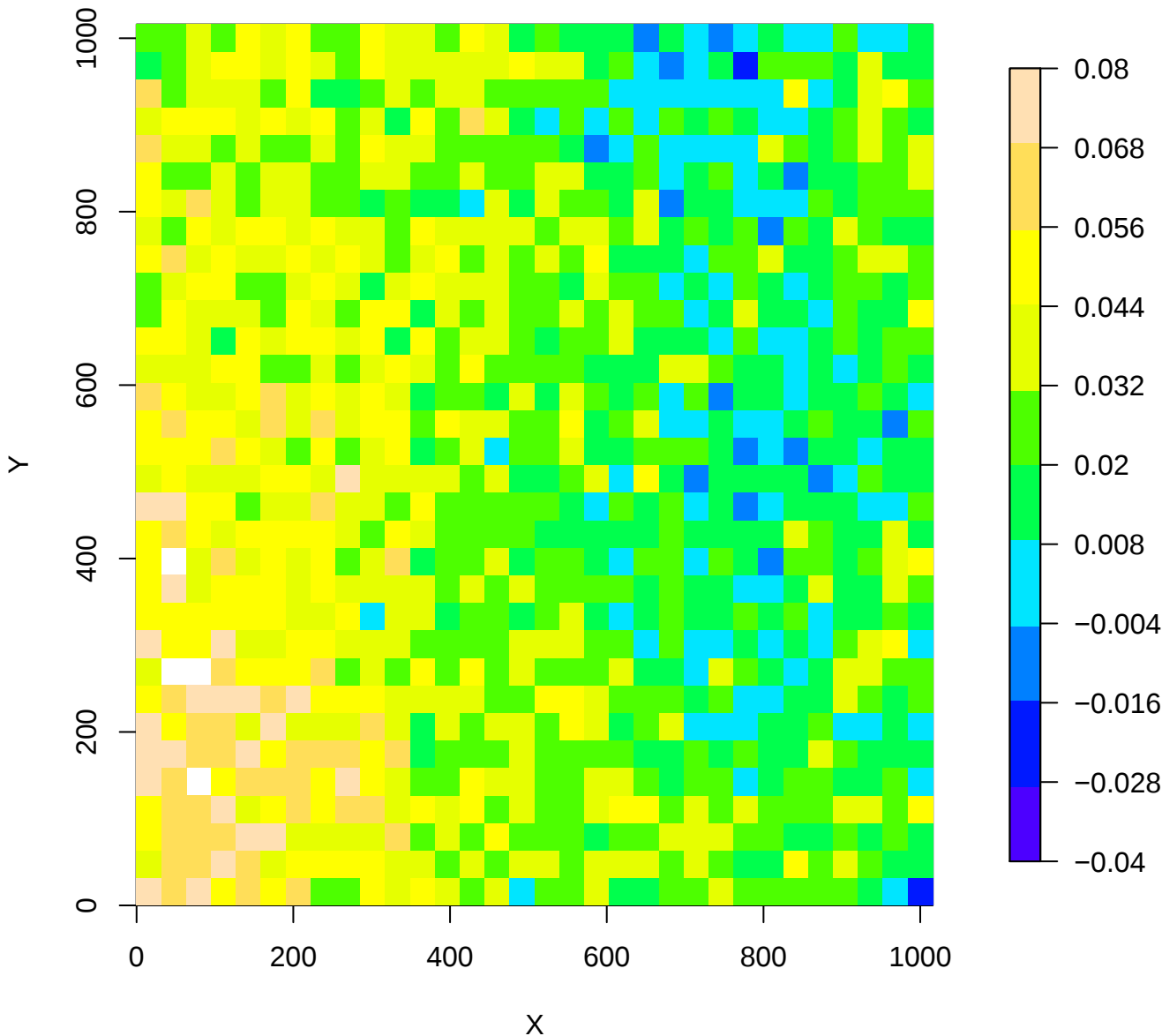
46940a POPS: binned median of "Ks - w2mpro" [mag]
