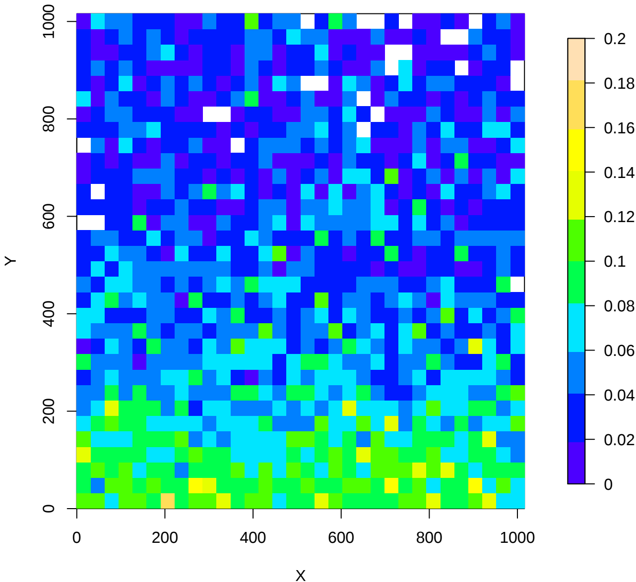
44525a: binned median of "Ks - w2mpro" [mag]
