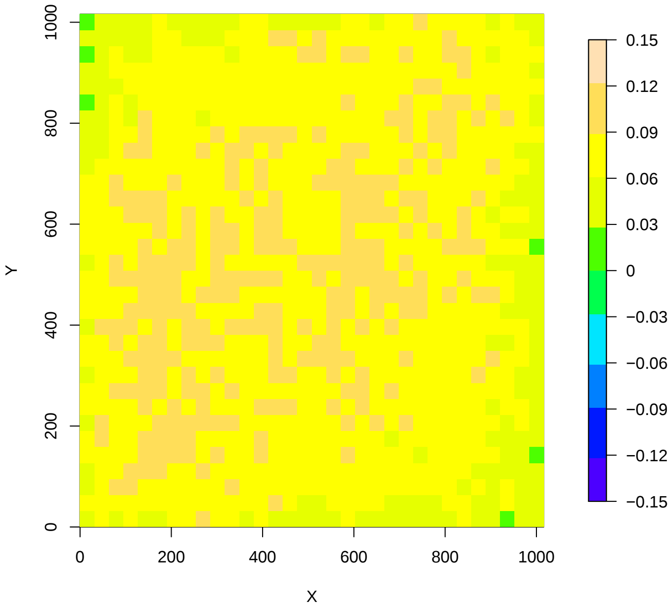
03750a OPS: binned median of "Ks - w1mpro" [mag]
