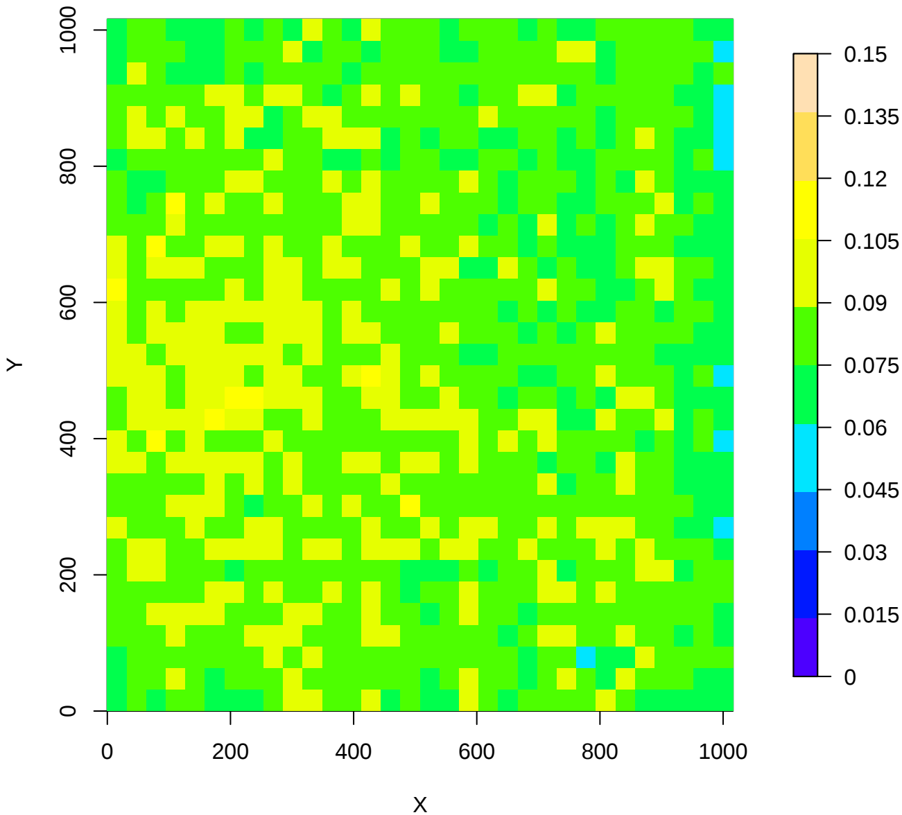
47222a POPS: binned median of "Ks - w1mpro" [mag]
