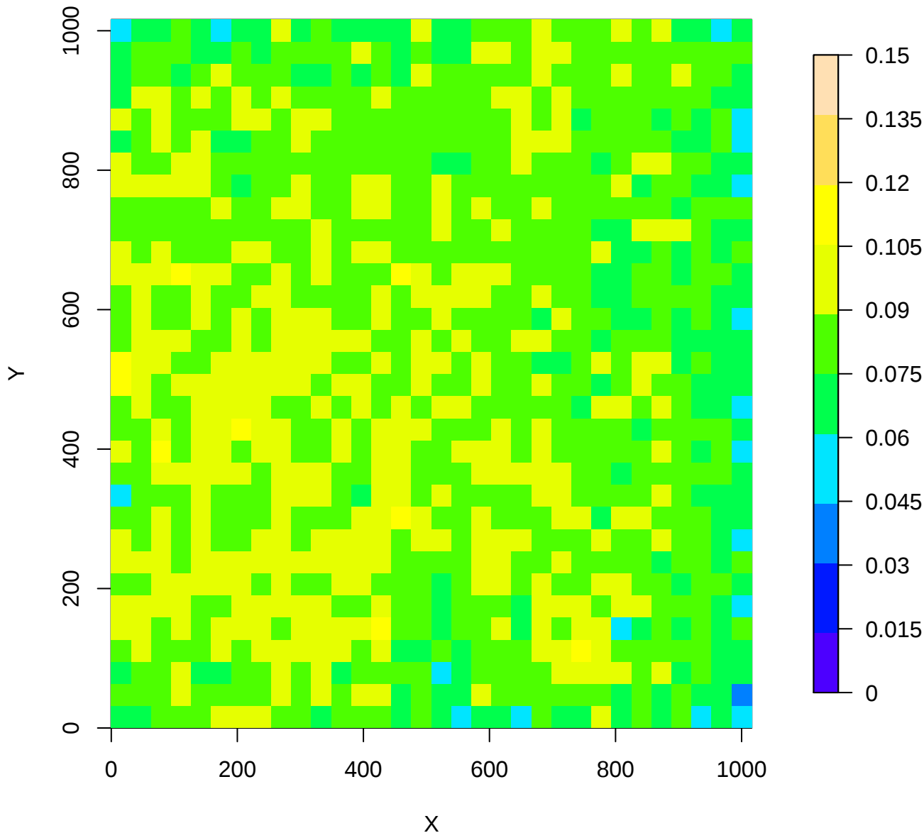
47585b POPS: binned median of "Ks - w1mpro" [mag]
