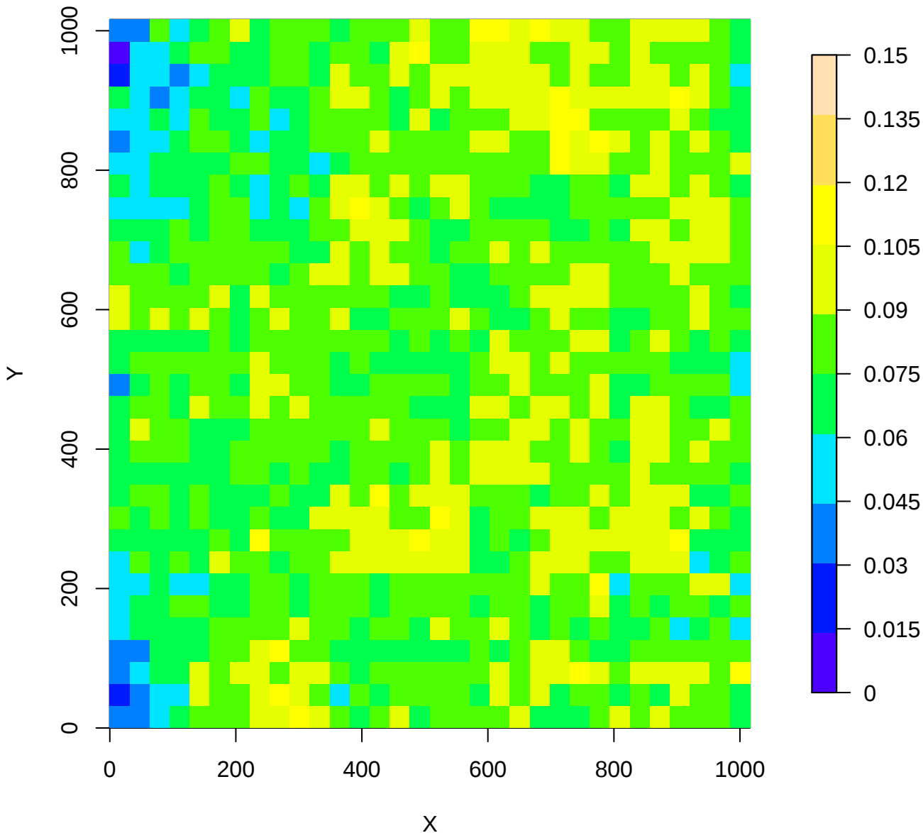
46940a OPS: binned median of "Ks - w1mpro" [mag]
