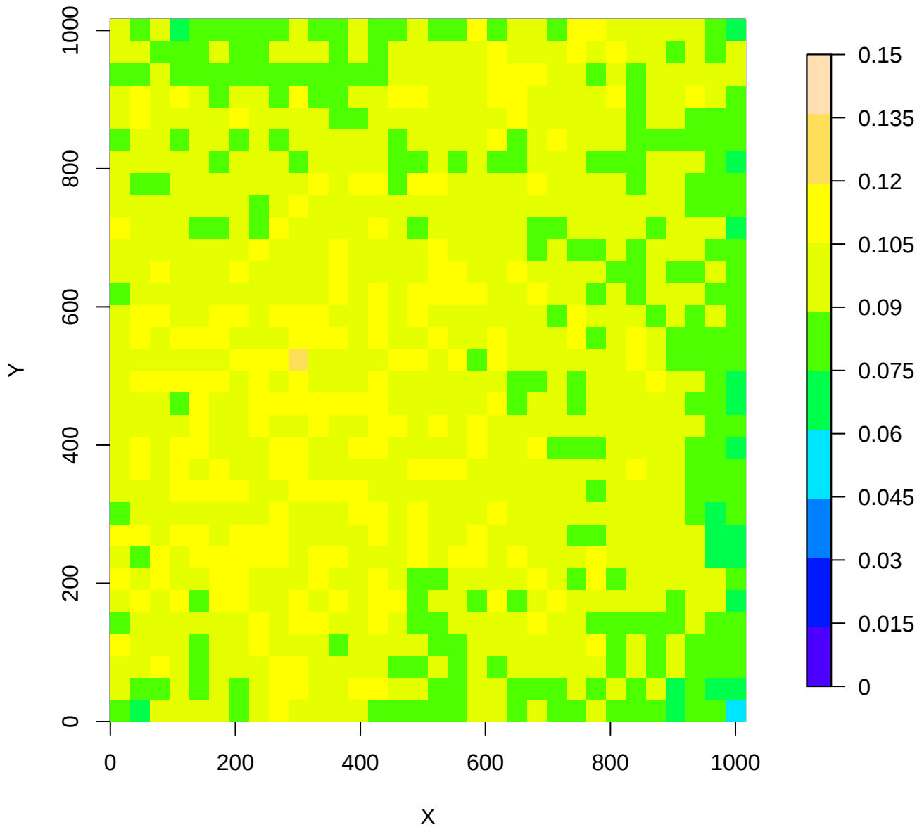
46938a: binned median of "Ks - w1mpro" [mag]
