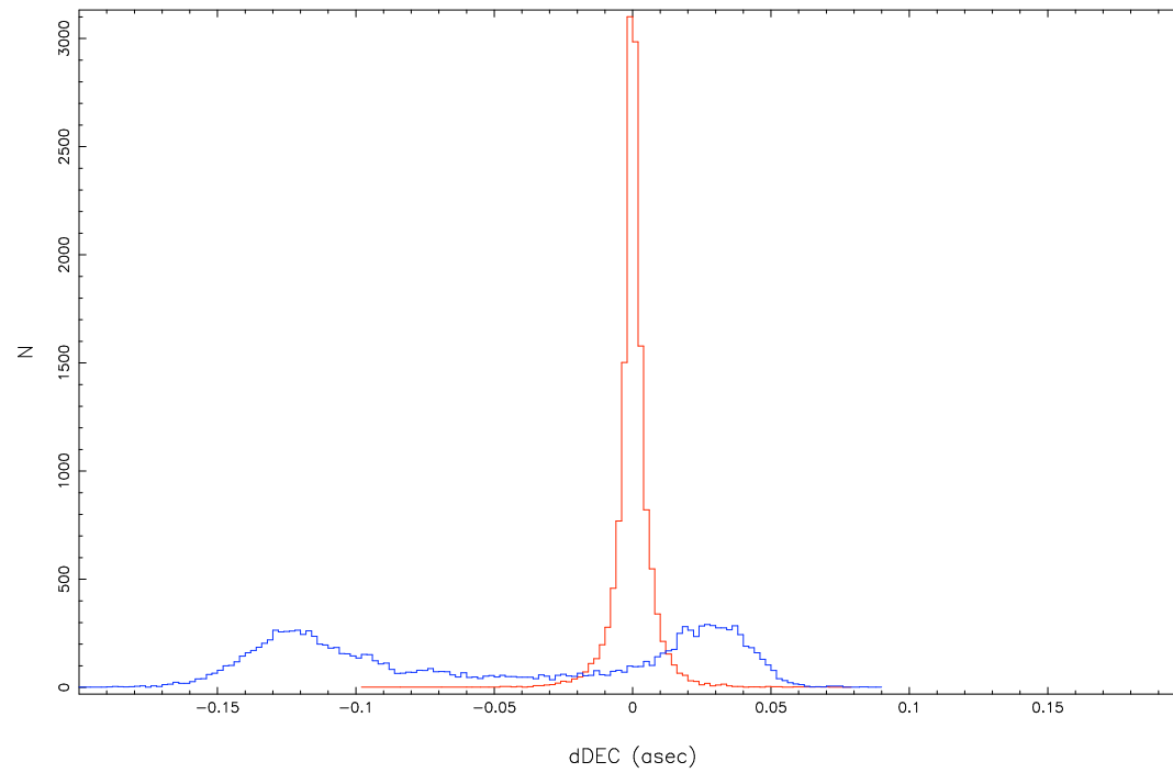
dDEC Histograms for SFMP20p-2MASS (red) & MDEX-SFMP3p (blue)
